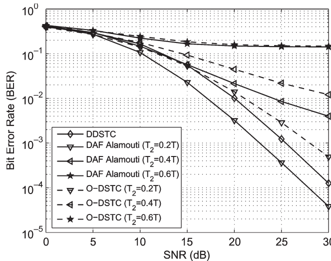
Fig. 6. BER performance with propagation delay mismatch. Two relay cases.
