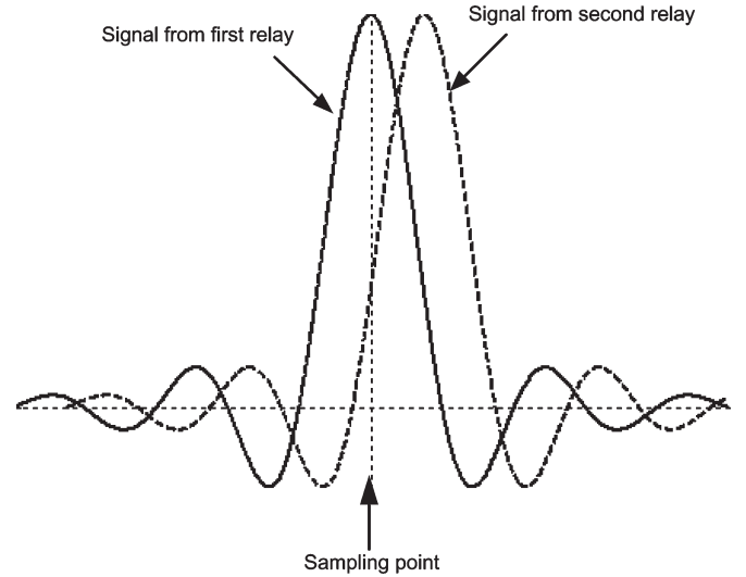
Fig. 3. Baseband signals (each is a raised-cosine pulse-shaped) from two relays at the receiver.
