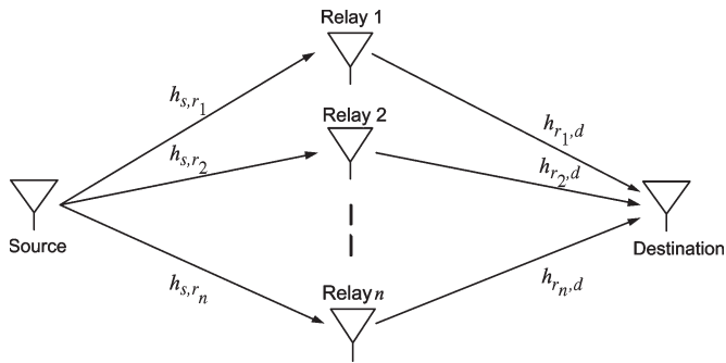
Fig. 1. Simplified system model for the two-hop distributed ST codes.
