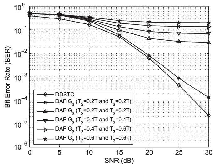
Fig. 7. BER performance with propagation delay mismatch. Three relay cases.
