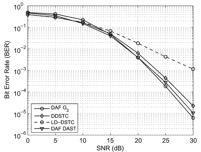
Fig. 5. BER for three relays with a data rate of 1 bit/sym.
