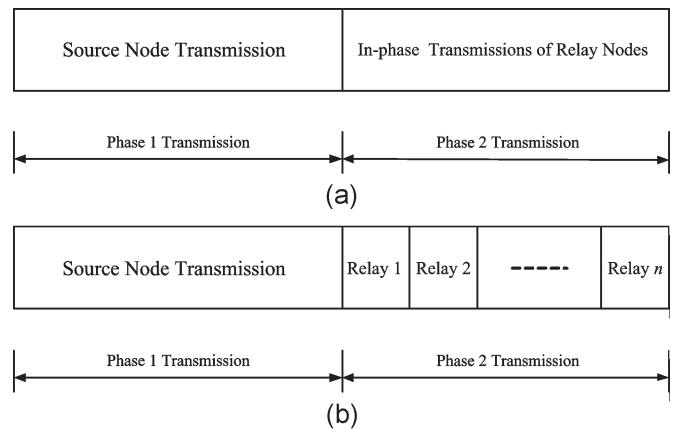
Fig. 2. Time frame structure for (a) conventional distributed ST codes and (b) DDSTCs.
