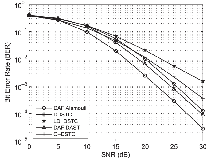
Fig. 4. BER for two relays with a data rate of 1 bit/sym.
