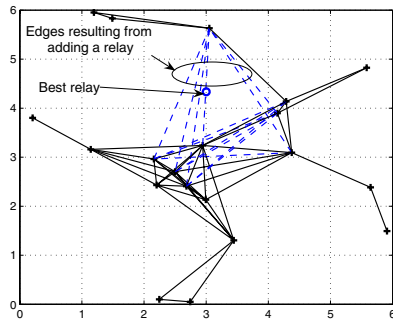
Fig. 1. Sensor network consisting of n = 20 nodes in a 6 \times 6 area. Sensors and relay are represented in + and o, respectively. Original and new edges are represented in solid and dashed lines respectively
