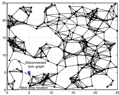
Fig. 5. Sensor network consisting of n = 200 nodes in a 25 \times 25 area. The network is reconnected by adding K = 1 relay at the location (4.98, 5.02) .
