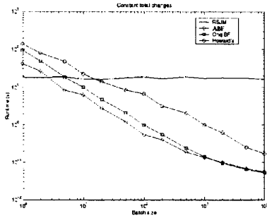
Figure 1: Comparison of algorithms as batch size varies
