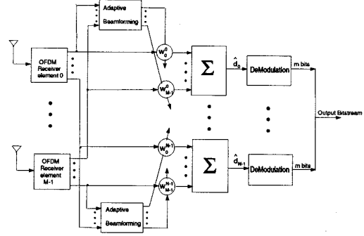
Figure 3. Antenna Array in an OFDM Receiver
