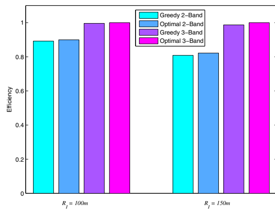
Fig. 4. Approximate efficiency of the greedy algorithm compared to the optimal solution.
